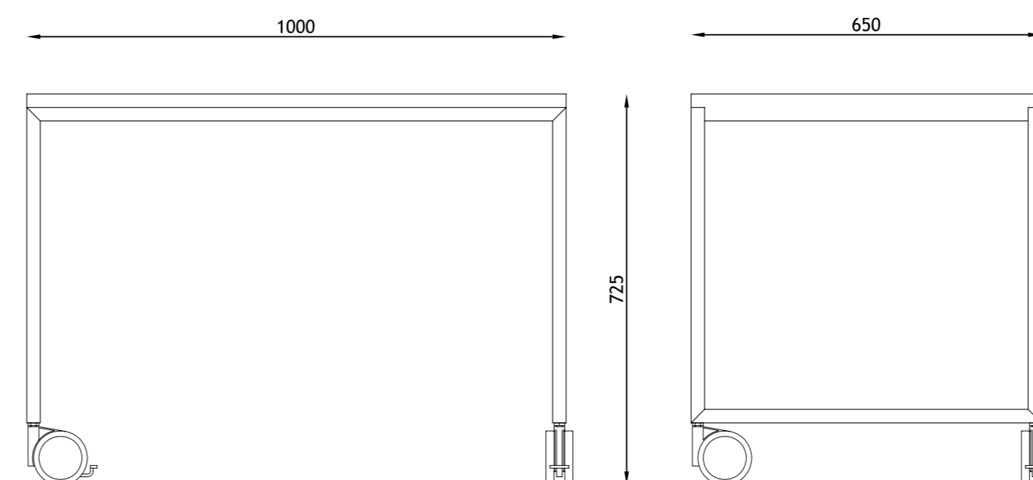
M3-212-000 MÓDUL 100-M/S (1000x650x725) OGTM ROLL.
