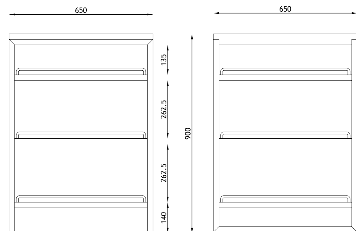
M3-230-000 MÓDUL 65 (650x650x900) SAFATES FIXES.
