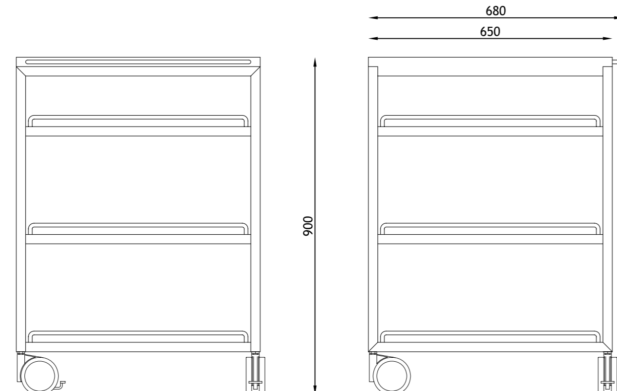
M3-231-000 MÓDUL 65-M (650x650x900) OGTM ROLL SAFATES FIXES.
