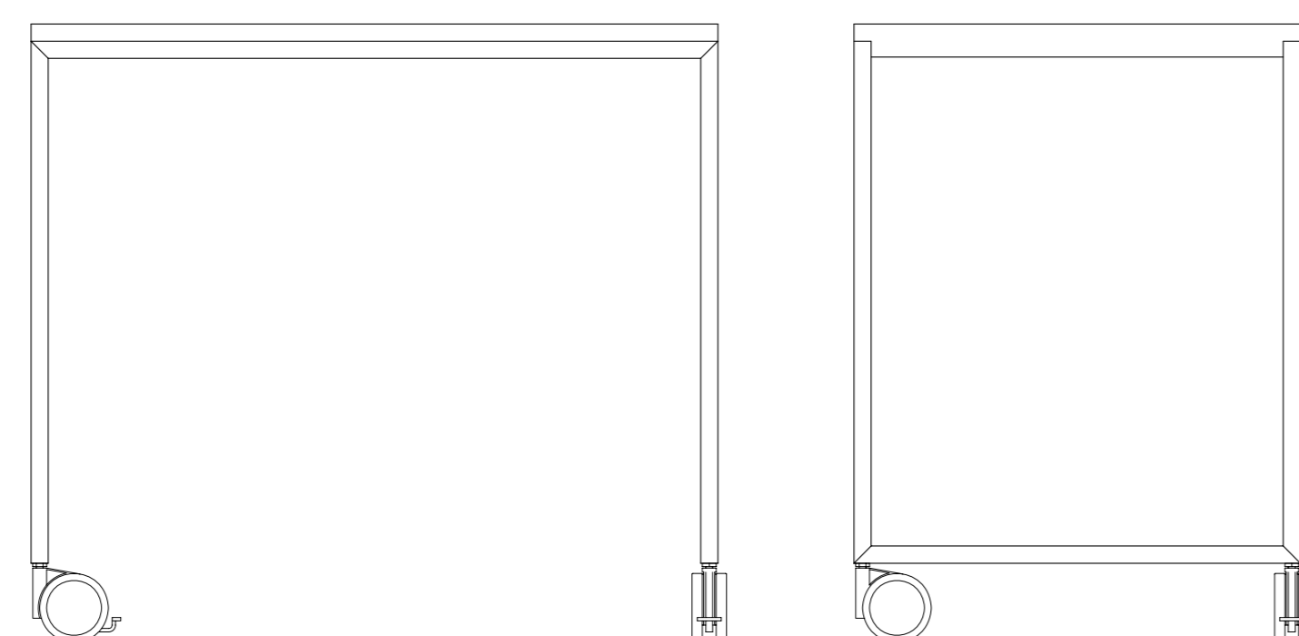
M3-211-000 MÓDUL 100-M (1000x650x900) OGTM ROLL.
