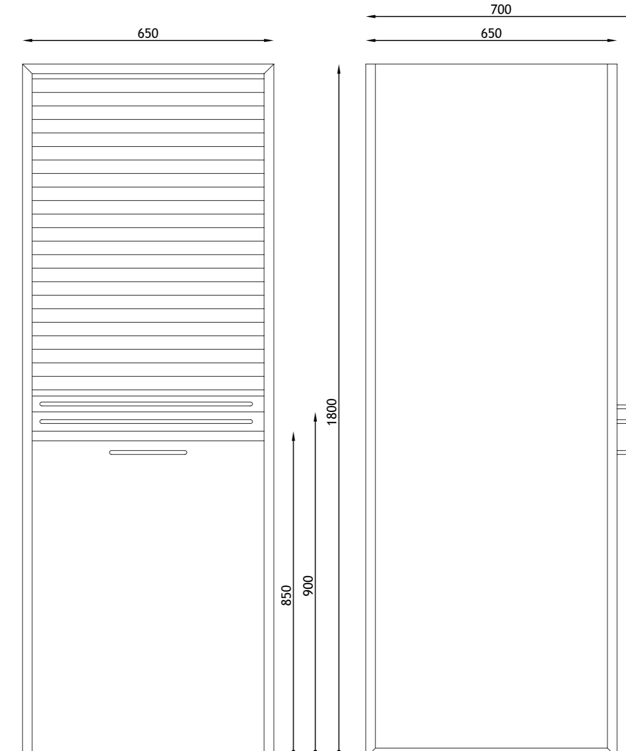
M3-260-000 MÓDUL 65-V (650x650x1800) RENTAVAJELLES SMEG STX1-J (600x600x850).
